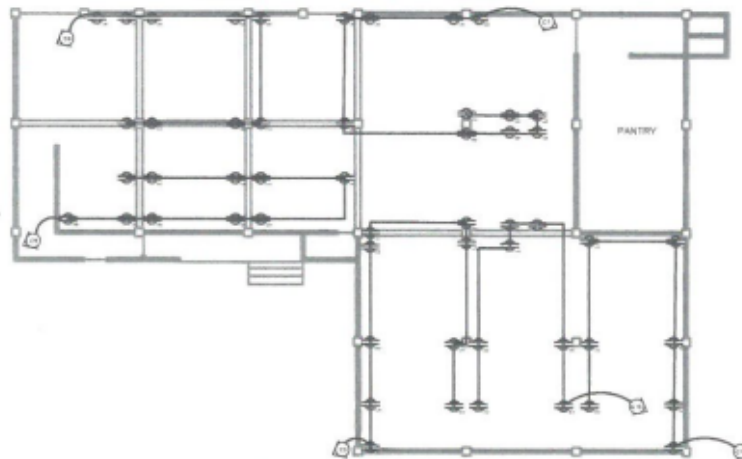
POWER LAYOUT PLAN
